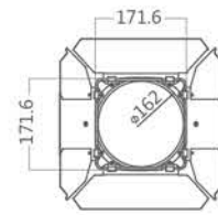
Barn doors (X40225)
