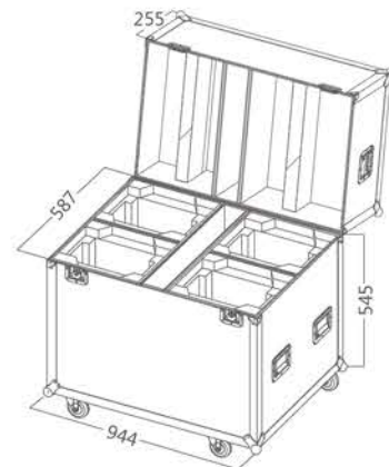
Flight Case (P20176)
