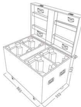
Flight Case (P20165)
