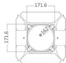
Barn doors (X40225)
