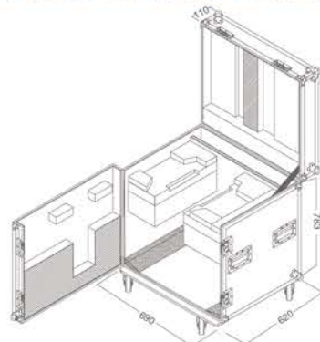
Flight Case ( P20227 )
