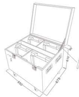
Flight Case (P20176)
