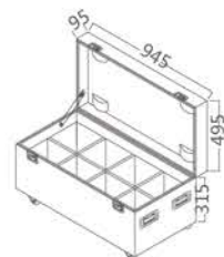
Flight case (P20014)
