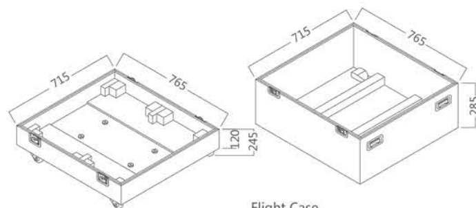
Flight Case (P20110)
